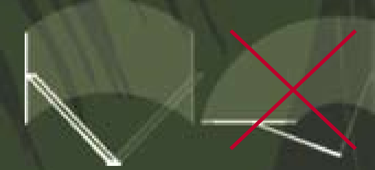
Pantographic Windshield Wipers (left) clean a wider swath of windshield than typical radial windshield wipers (right) of similar blade length.
